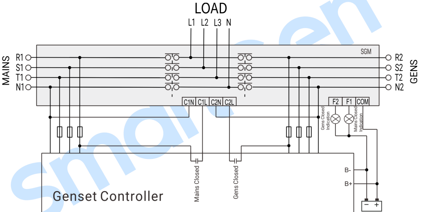
Fig.5 - SGM (Genset) Wiring Connection
