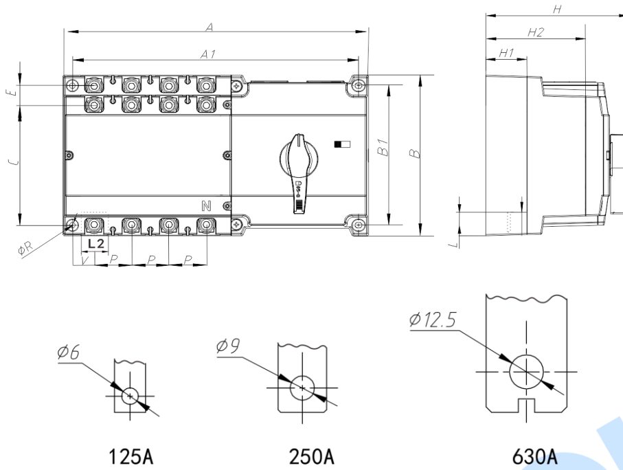
Fig.2 - SGM/SGMA-125A/250A/630A Shell Frame
