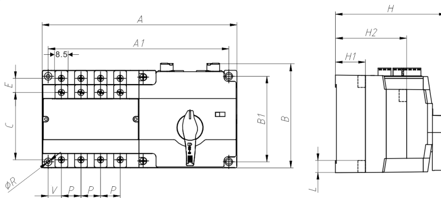
Fig.1 - SGM/SGMA-80A Shell Frame
