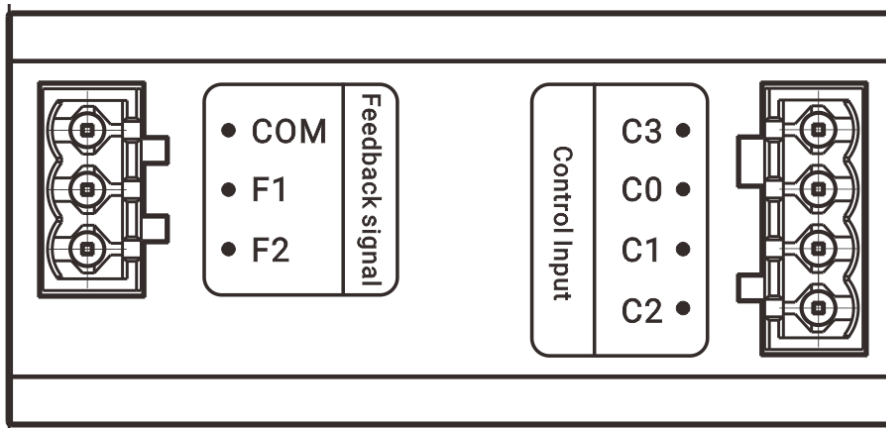
Fig.4 - SGMA Series Terminal
