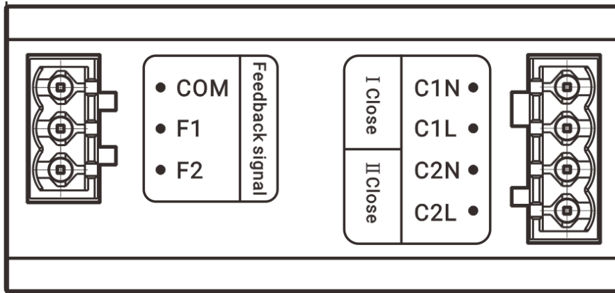
Fig.3 - SGM Series Terminal
