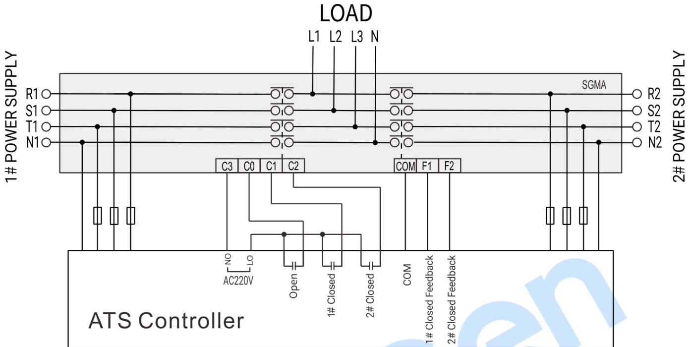
Fig.6 - SGMA (ATS) Wiring Connection
