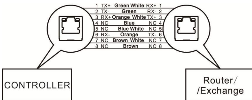
Fig.12 – Direct Connection Between Controller and Router
