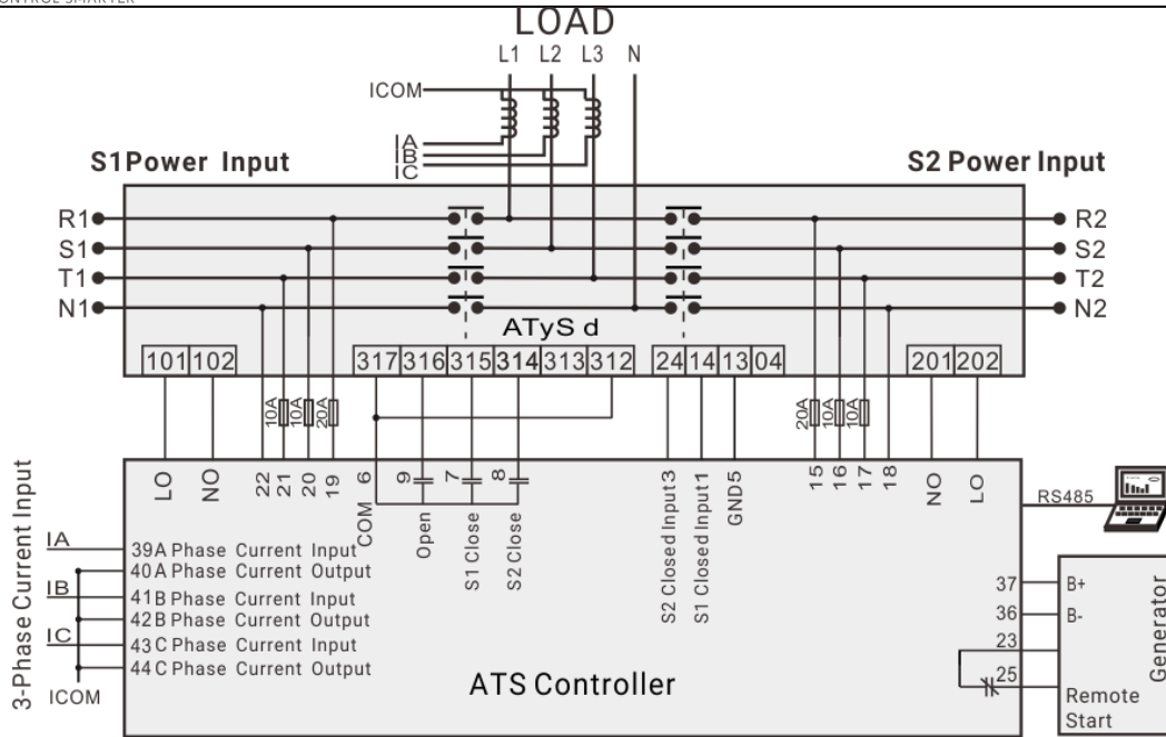
Fig. 20 – AtySd Application Diagram
