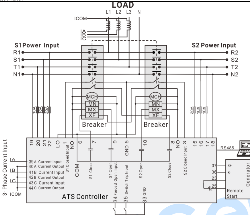
Fig. 23 – Breaker Application Diagram
