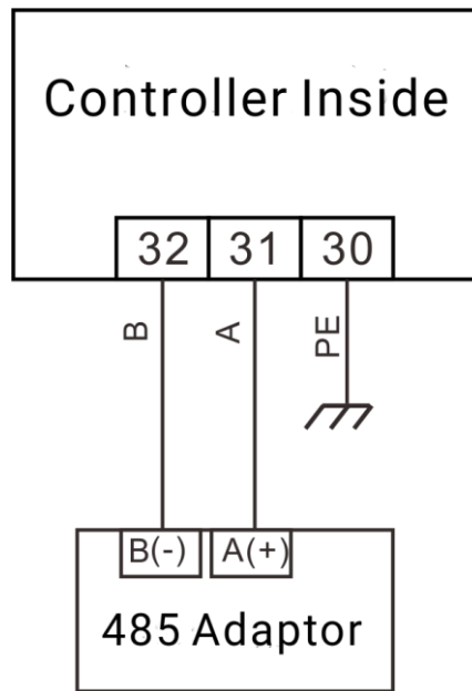
Fig. 17 – RS485 Connection
