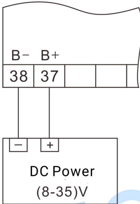
Fig. 15 – DC Supply
