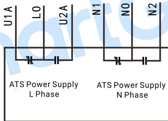
Fig. 9 – ATS Power Phase Voltage Supply
