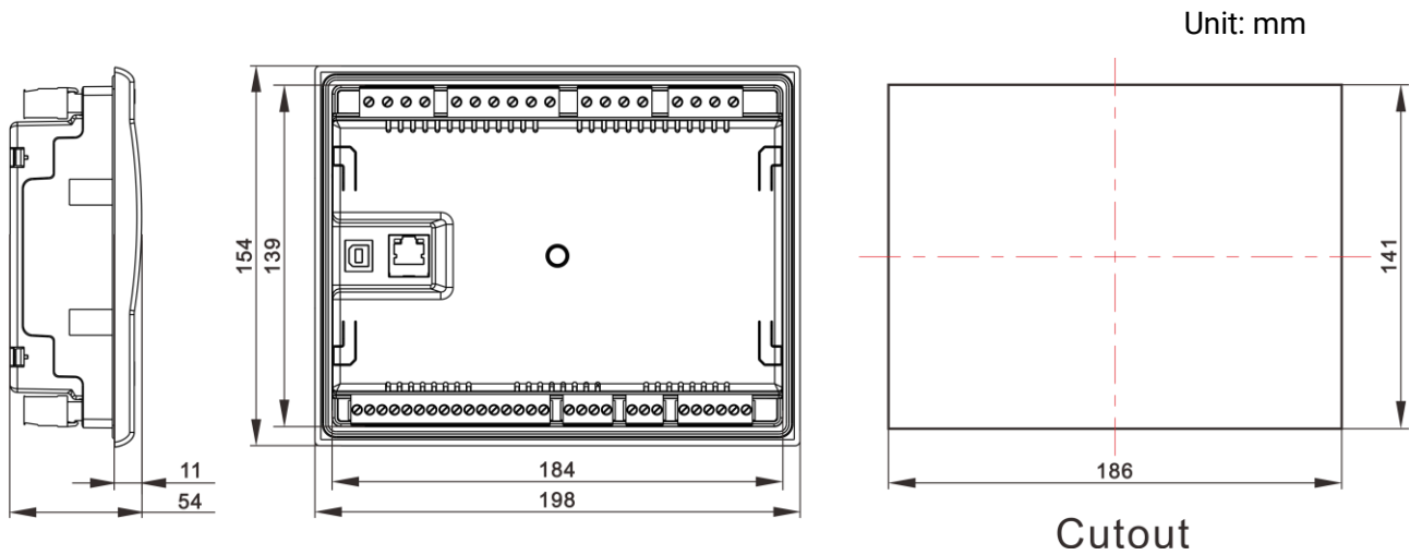
Fig. 24 – Case Dimensions and Panel Cutout
