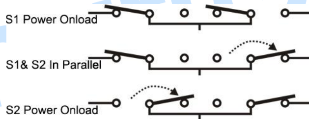
Fig. 6 – Sync Transfer Diagram
