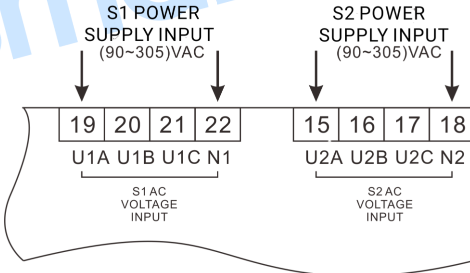
Fig. 16 – AC Supply
