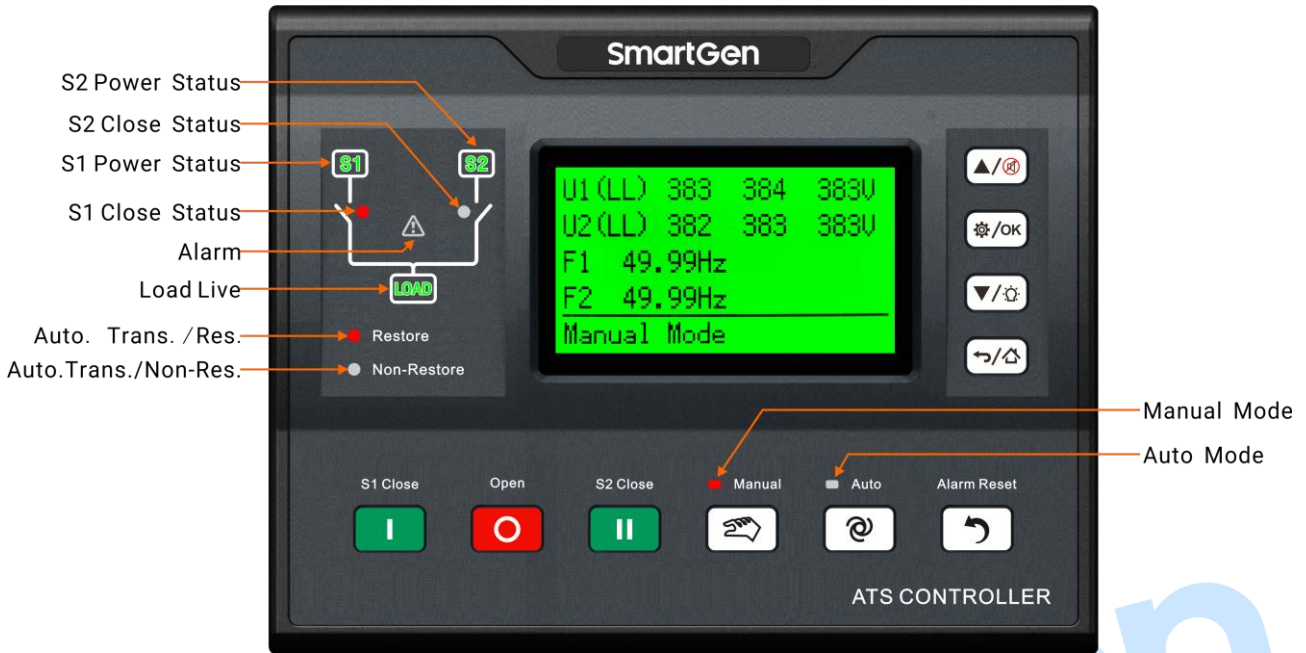
Fig. 2 – Front Panel
