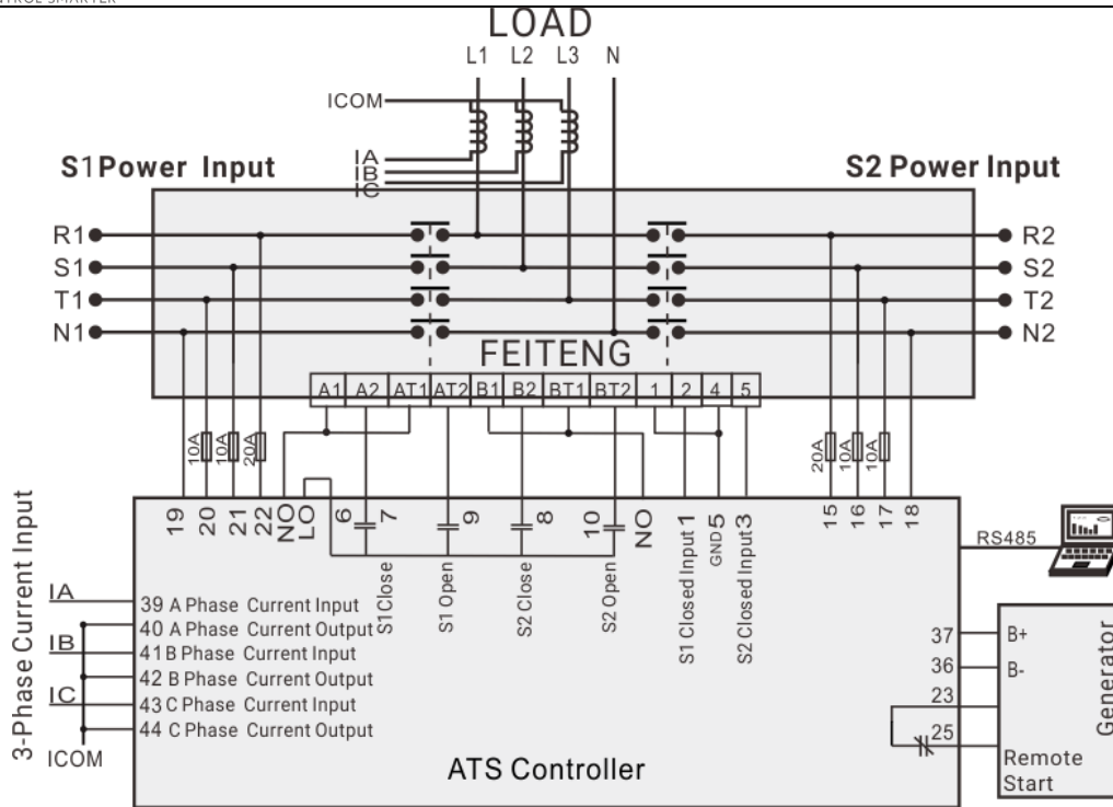
Fig. 21 – FEITENG Application Diagram
