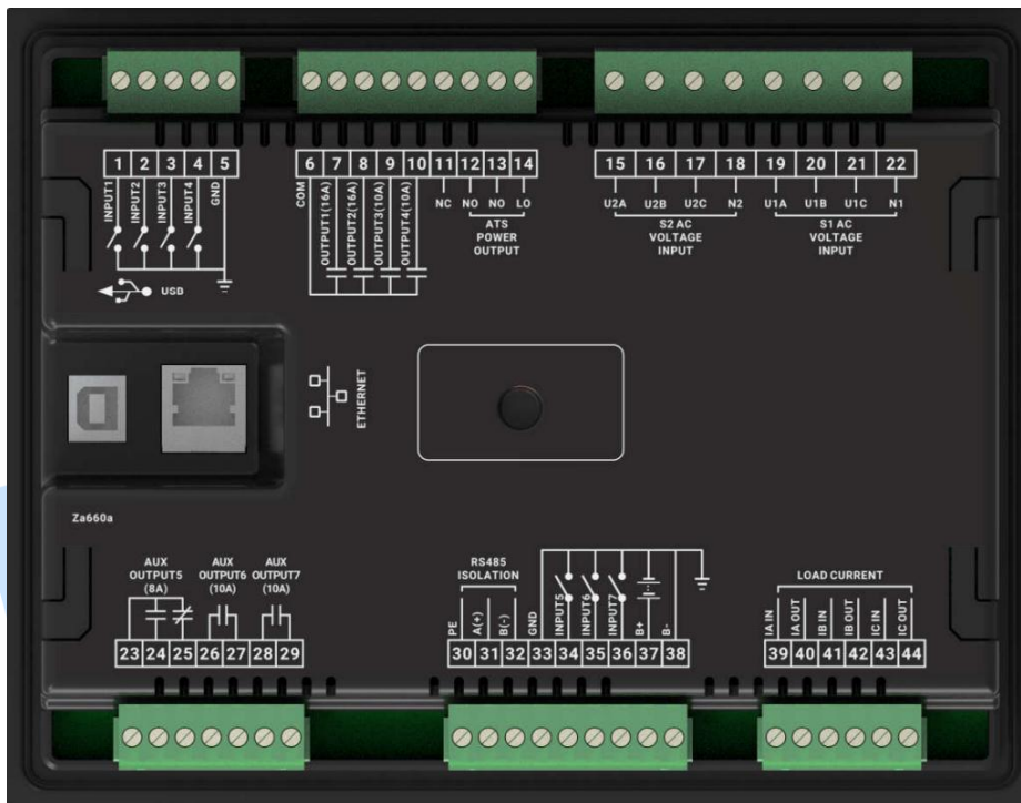
Fig. 14 – Controller Back Panel
