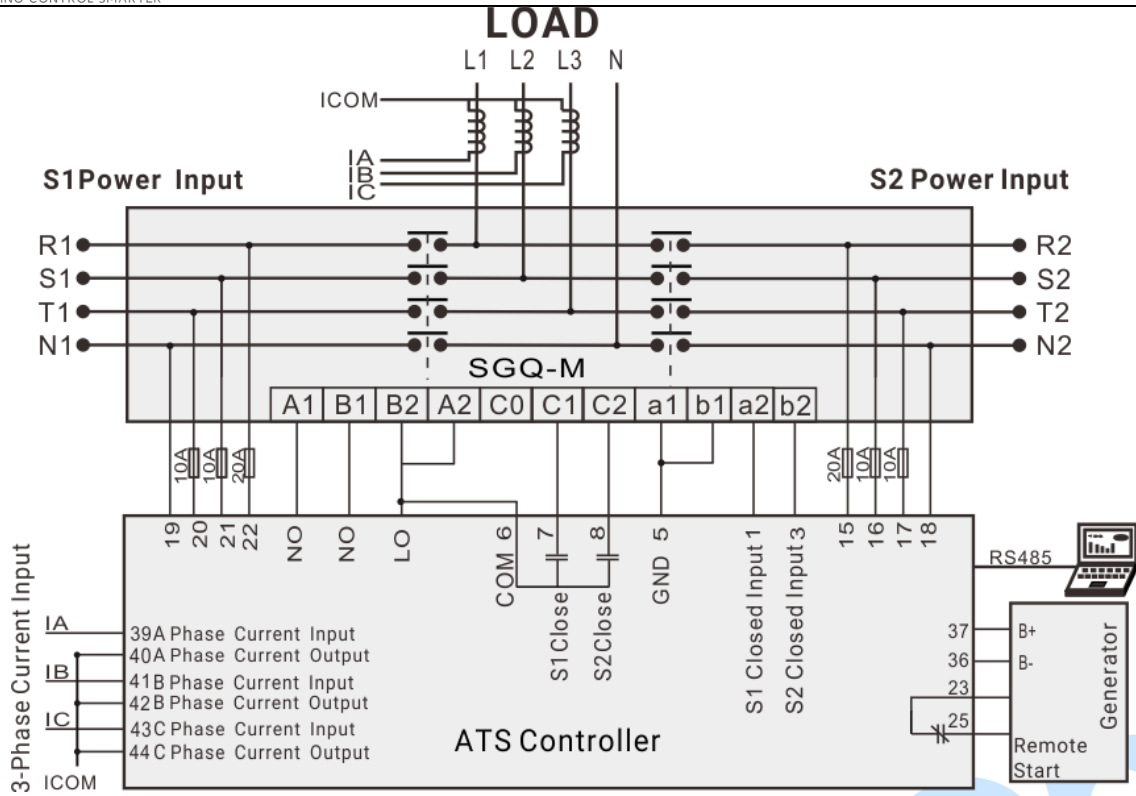
Fig. 19 – SGQ-M Application Diagram
