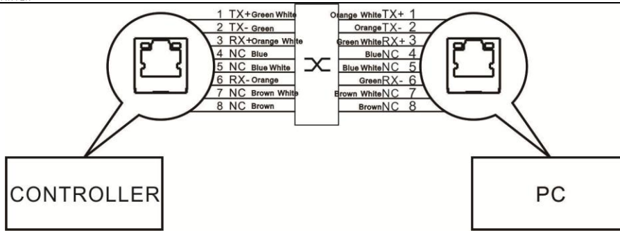
Fig. 13 – Cross Connection Between Controller and PC
