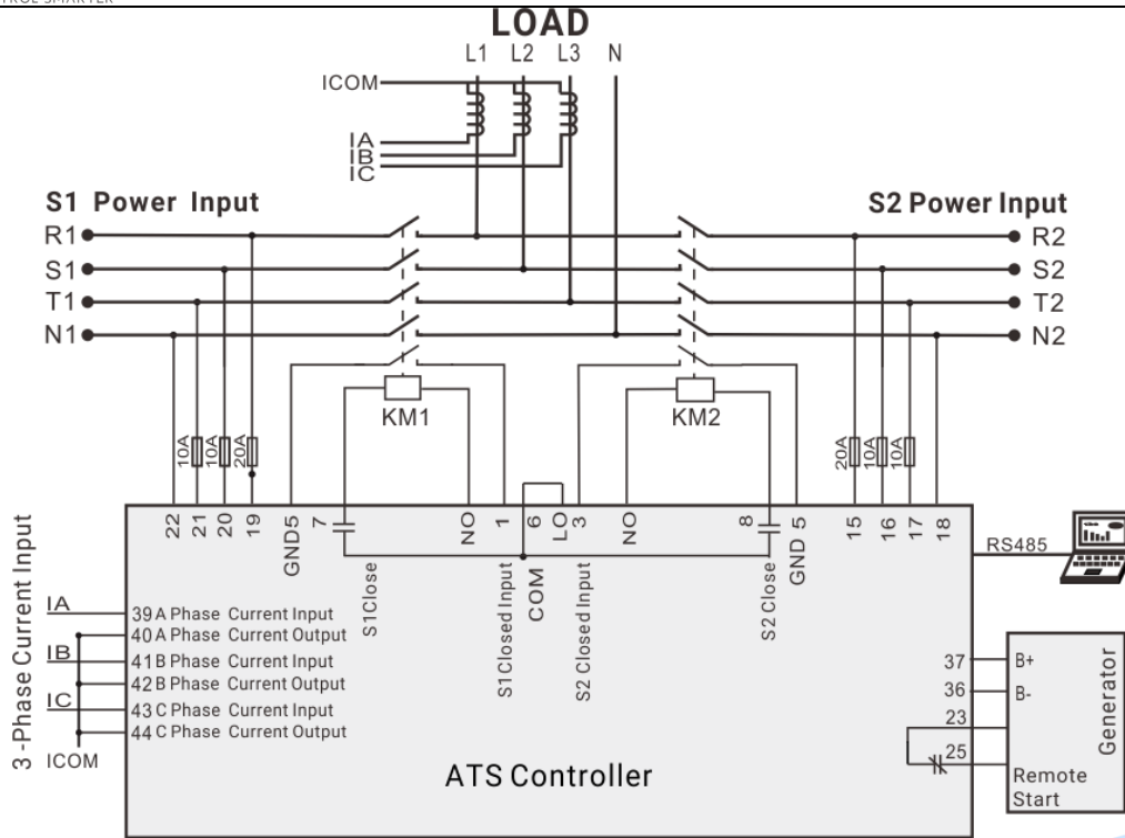
Fig. 22 – Contactor Application Diagram
