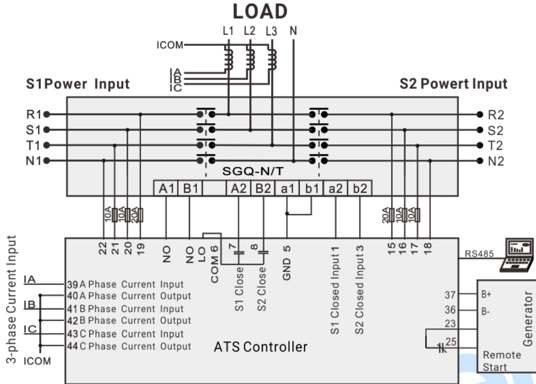
Fig. 18 – SGQ-N/T Application Diagram
