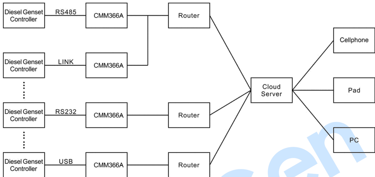
Fig.12 CMM366A-4G System Diagram
