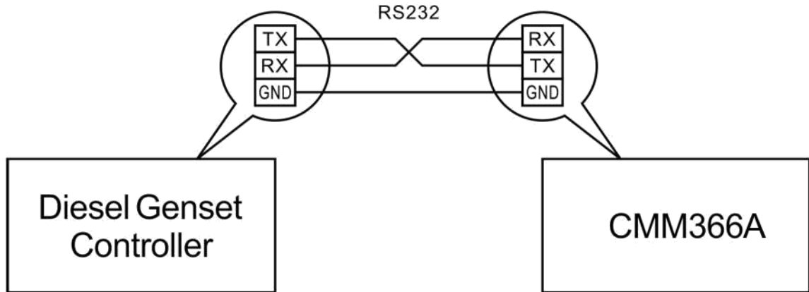
Fig.6 RS232 Connection
