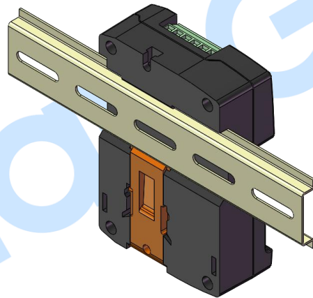
Fig.14 CMM366A-4G Guide Rail Installation
