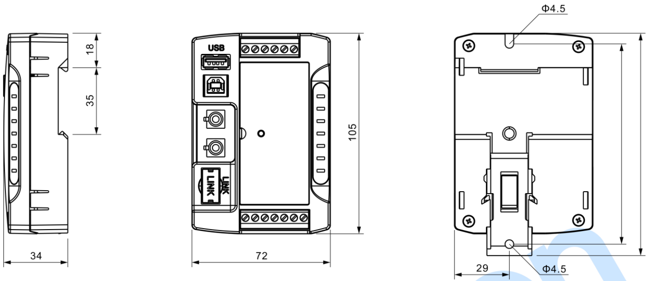
Fig.13 CMM366A-4G Case Dimension
