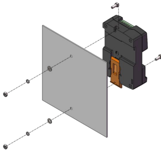
Fig.15 CMM366A-4G Screw Installation
