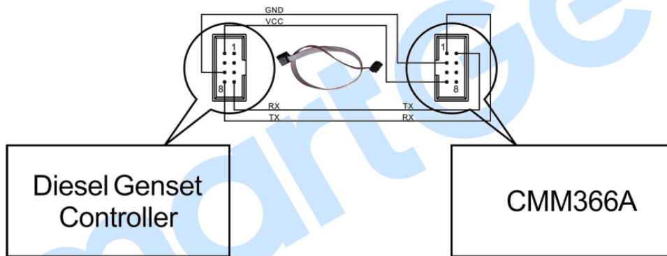
Fig.7 LINK Connection
