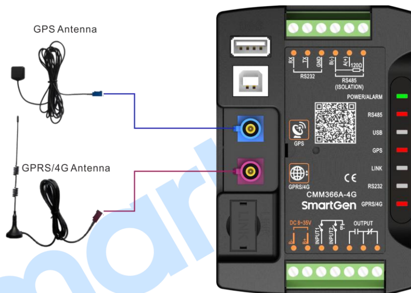
Fig.2 CMM366A-4G Antenna Connection
