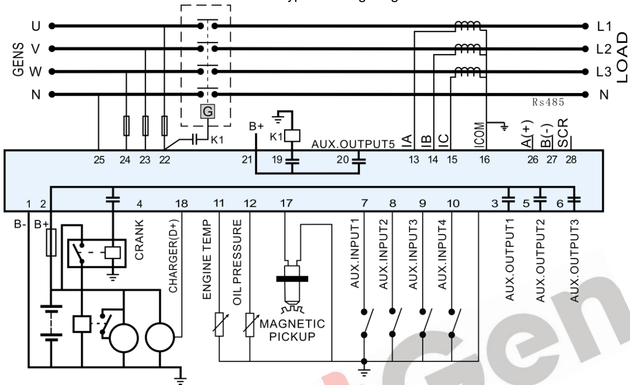
HGM410C Typical Wiring Diagram
