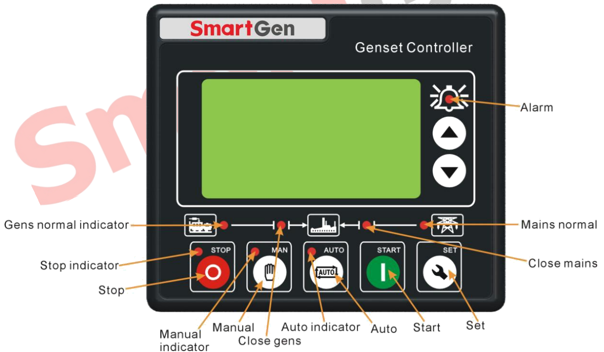
HGM420LT Panel Indicators
