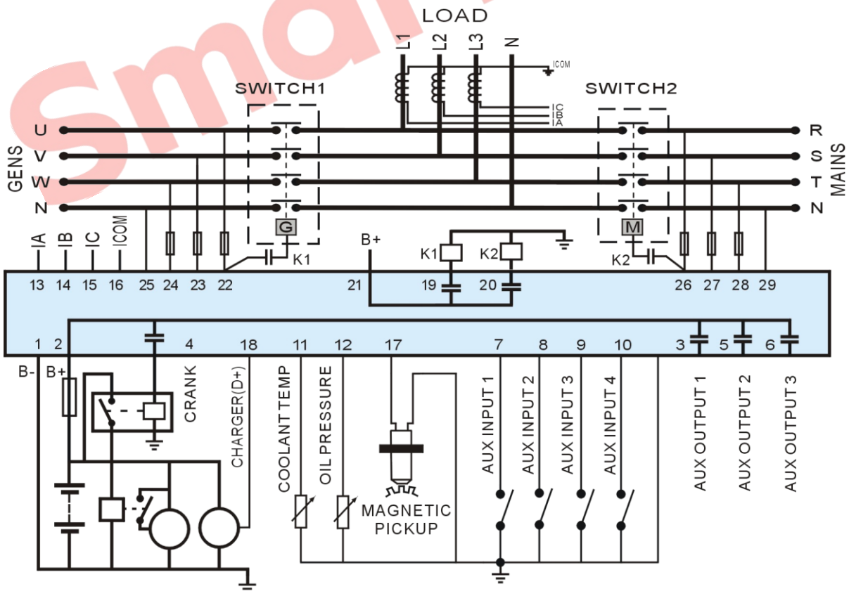
HGM420LT Typical wiring diagram
