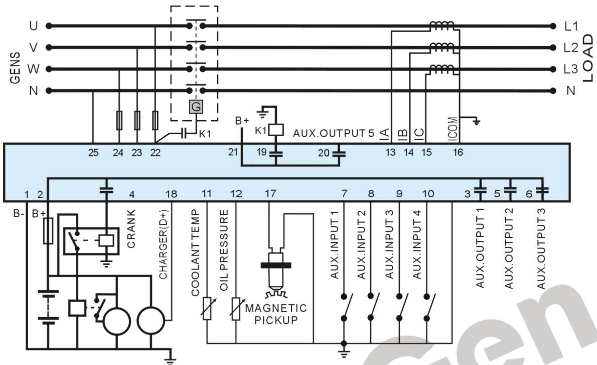
HGM410LT Typical wiring diagram
