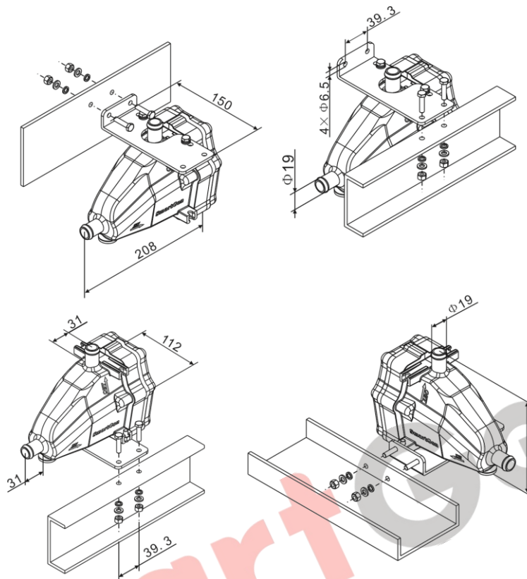
Fig.4 – Installation Dimensions
