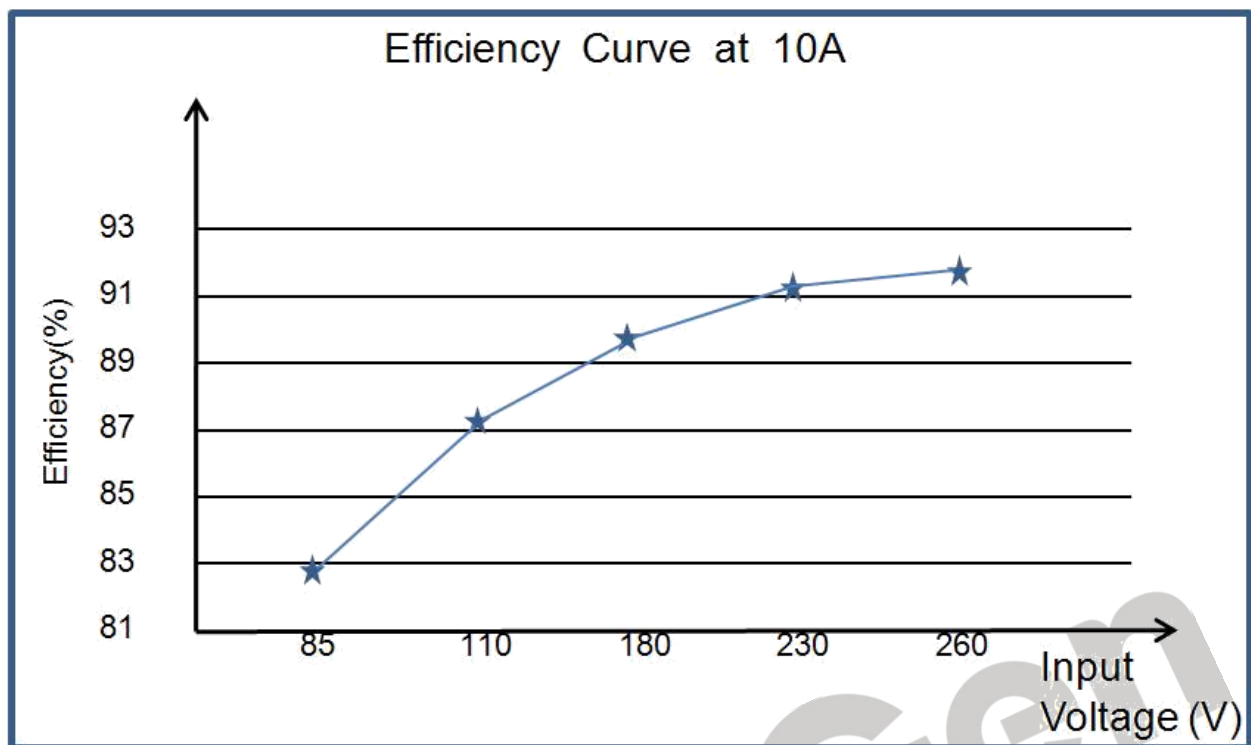
Fig.3 Efficiency Curve
