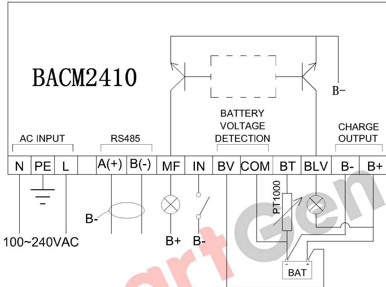
Fig.5 Connection Diagram
